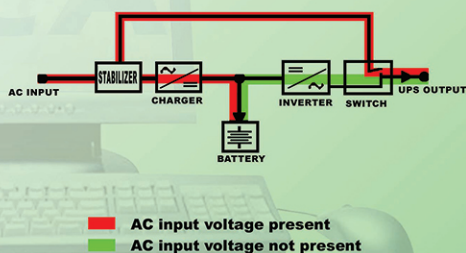
UPS DIAGRAM
